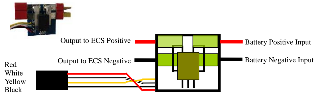
Figure3. Current Sensor
